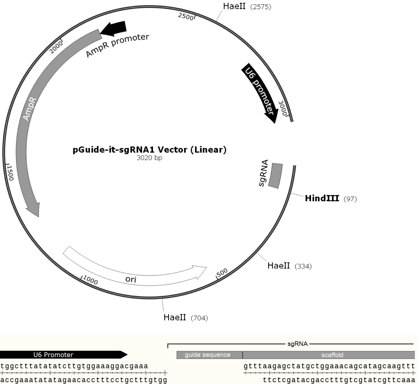
Figure 1. pGuide-it-sgRNA1 Vector (Linear) map and cloning site for user's guide sequence.
