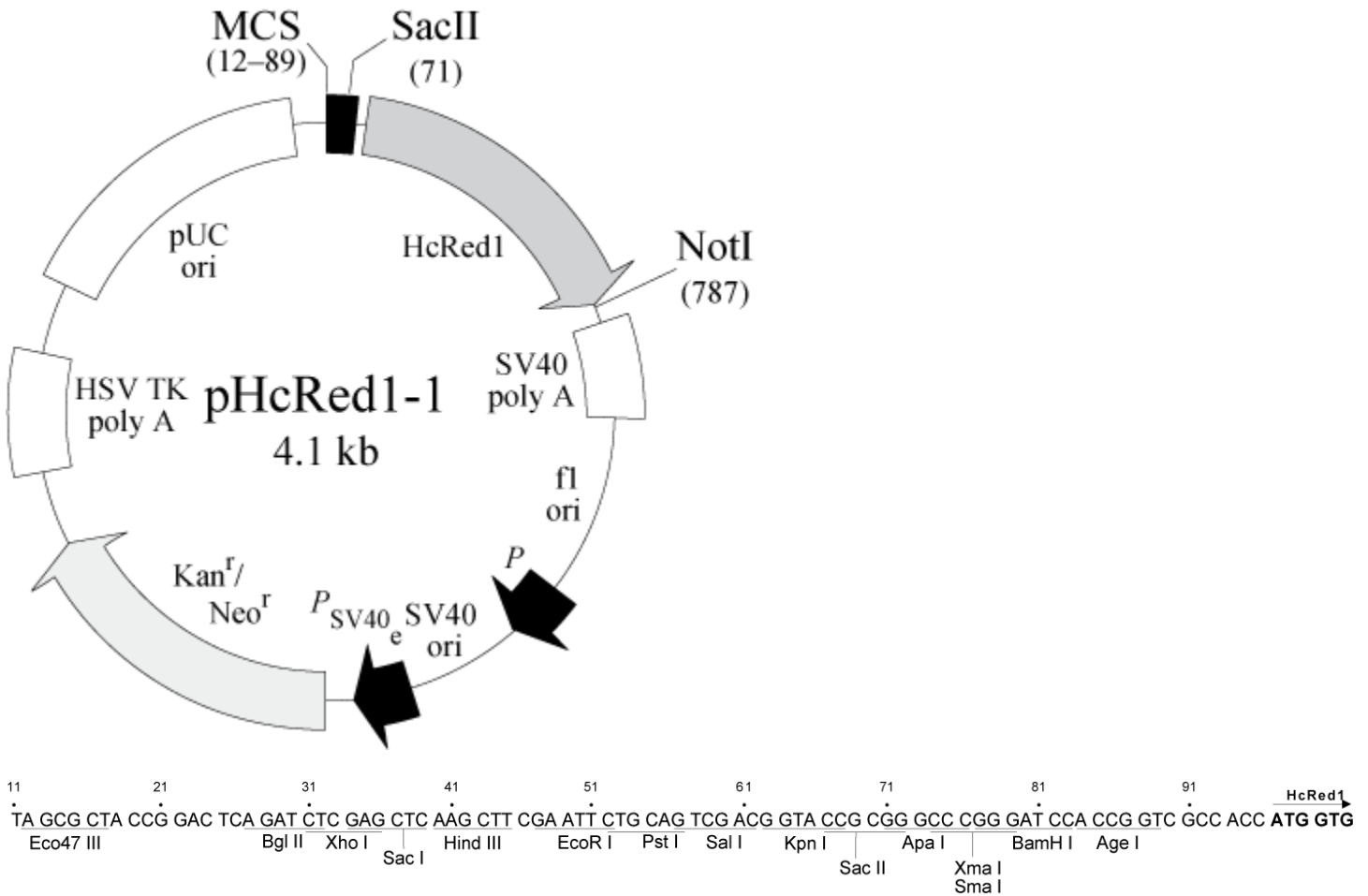
pHcRed1-1 vector map and multiple cloning site.
